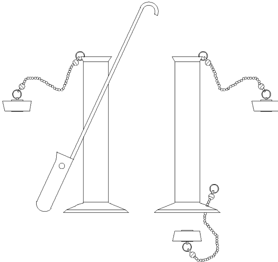
CLOSED BOTTOM
